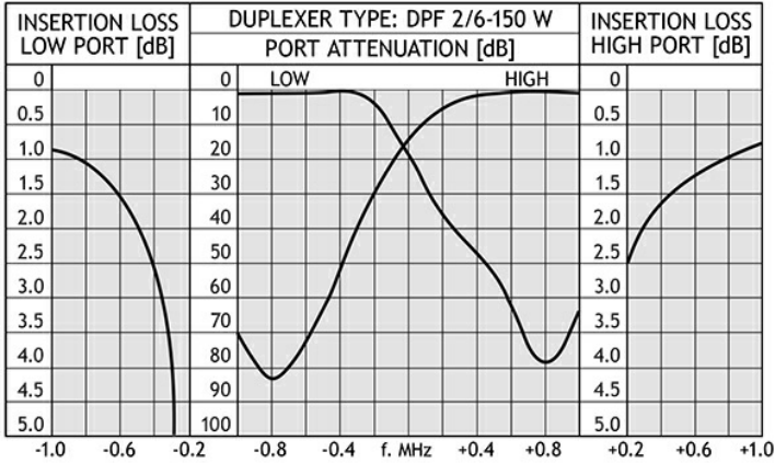
TYPICAL RESPONSE CURVES @ 1.6 MHZ DUPLEX SPACING
