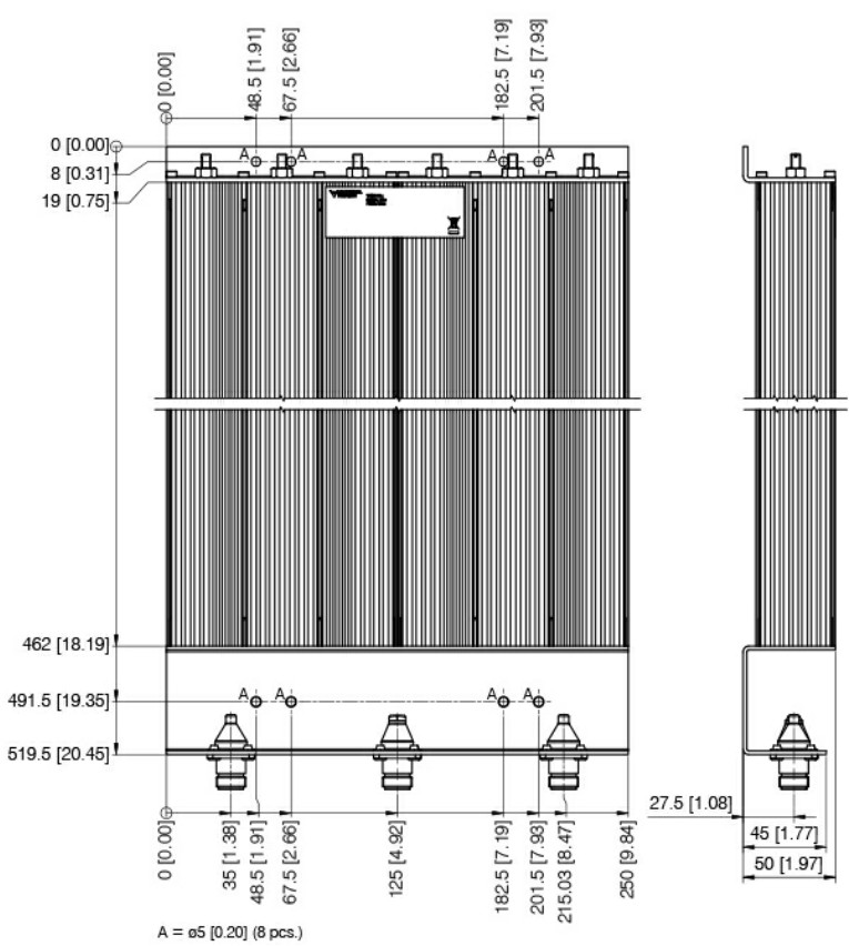
MOUNTING DETAILS
