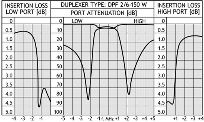
TYPICAL RESPONSE CURVES @ 4.5 MHZ DUPLEX SPACING
